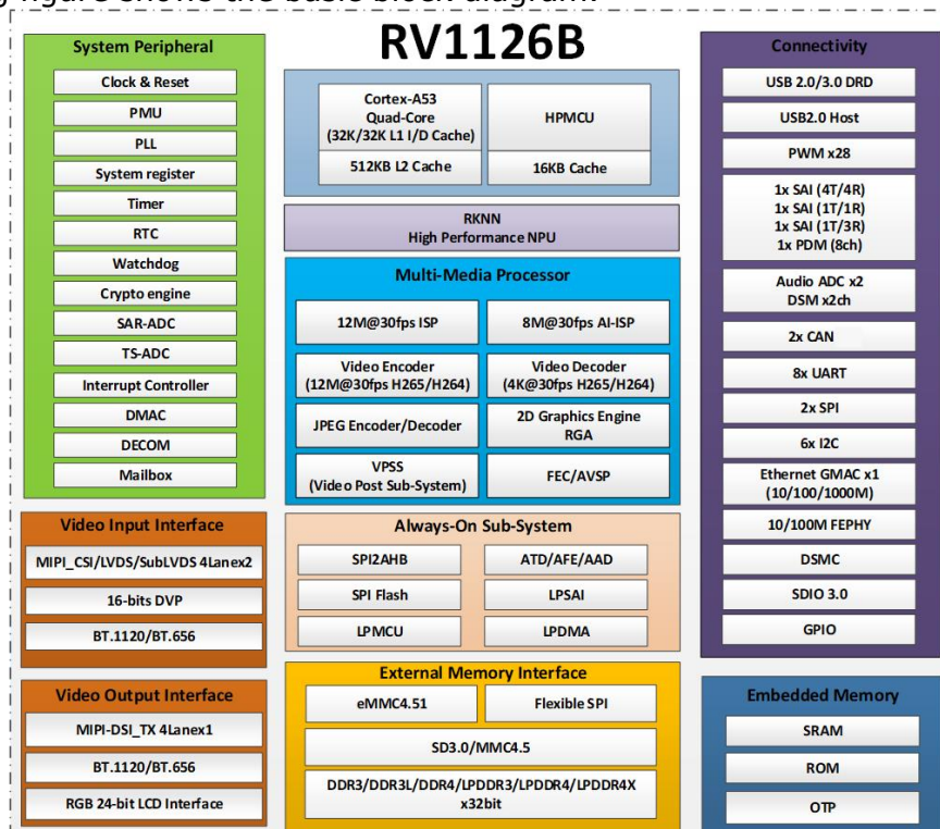
Fig. 1-1 Block Diagram
